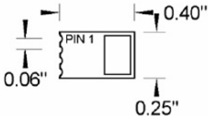
Figure 2: Mechanical Drawing for RCT-433-AS
