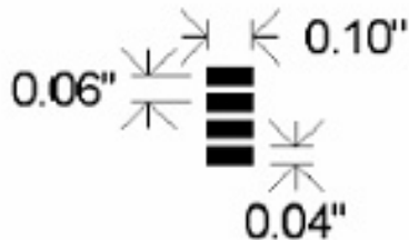
Figure 3: Suggested Pad Layout
